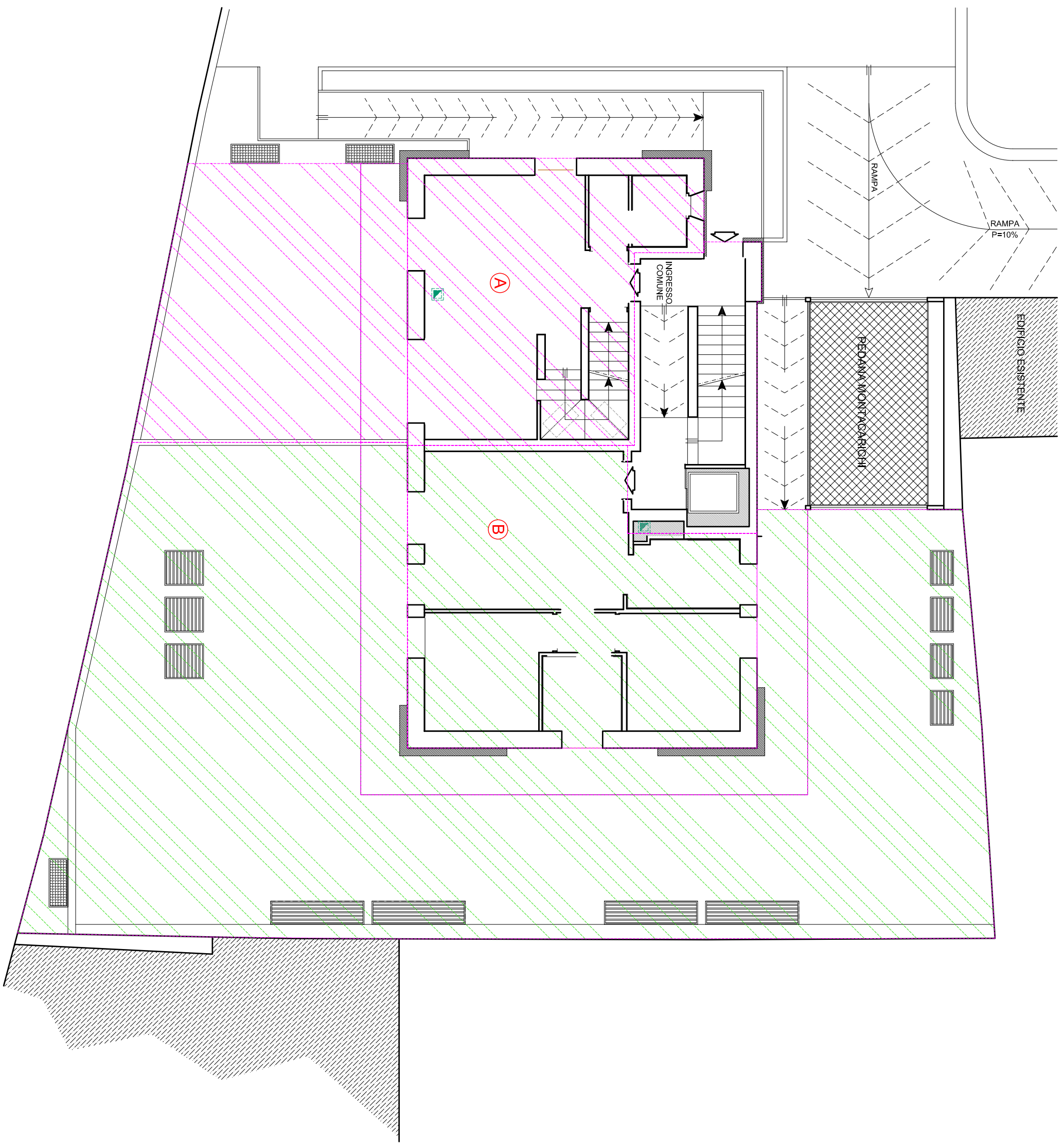
PIANTA PIANO TERRA H=279/255
